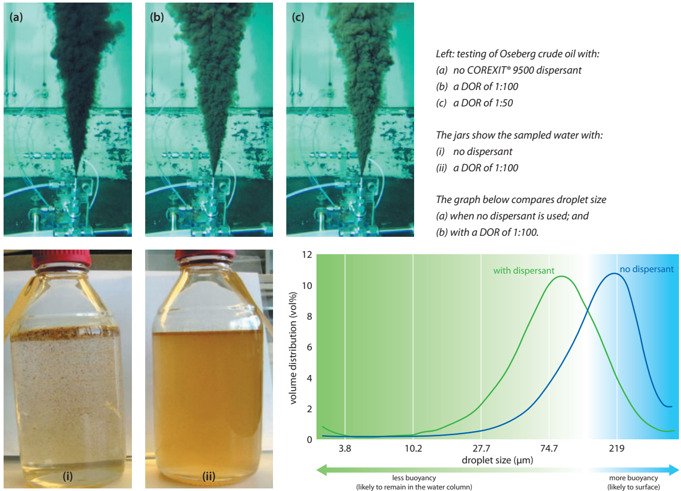
Figure 9 Testing of Oseberg crude oil with, and without, dispersant added (source: SINTEF)
