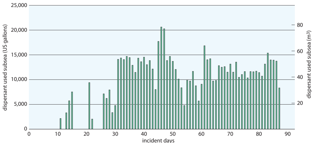
Figure 6 Dispersant application subsea during the Macondo incident
