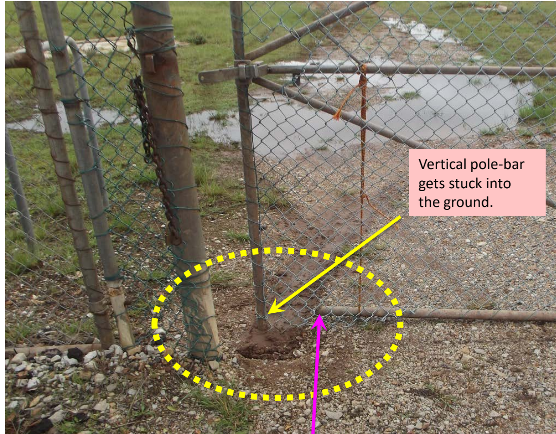
Bottom stiffener pole-bar of wire fence gate has rusted off.
