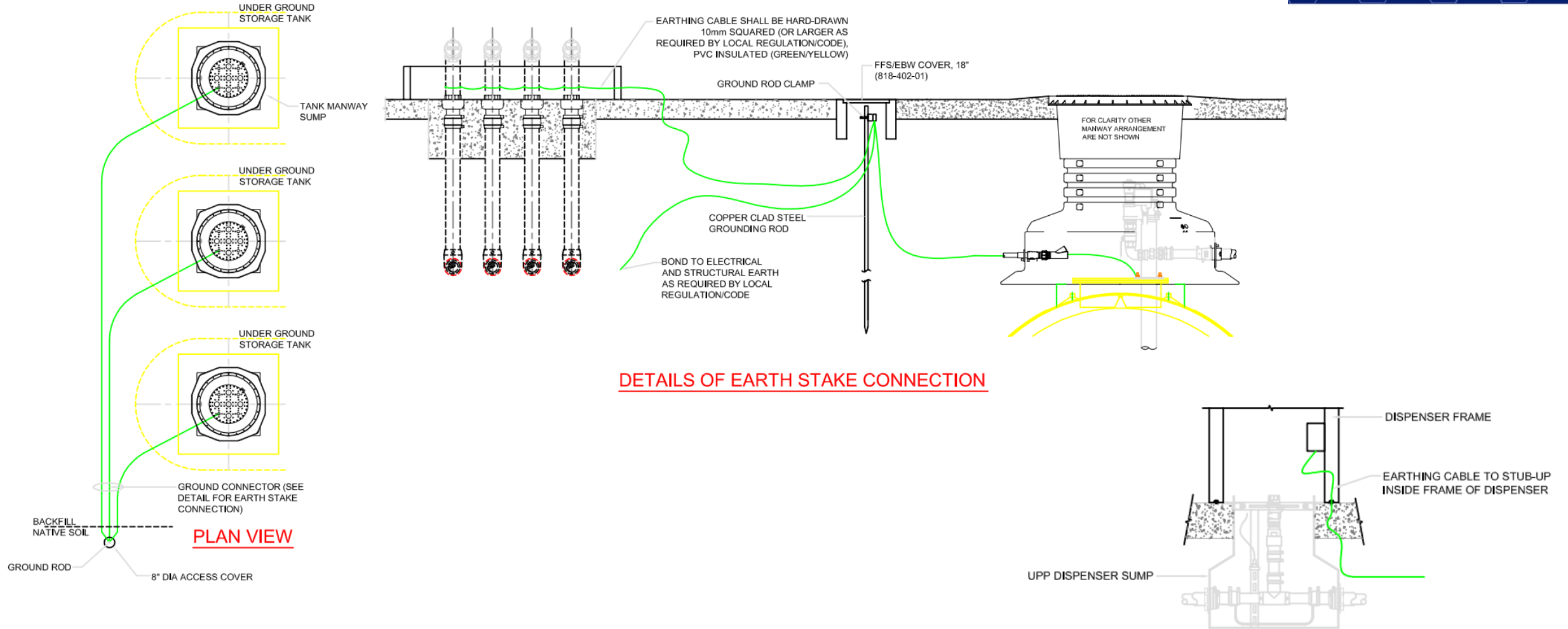
DETAILS OF DISPENSER SUMP EARTHING
