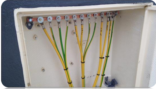
Grounding/Earthing of all Equipment
