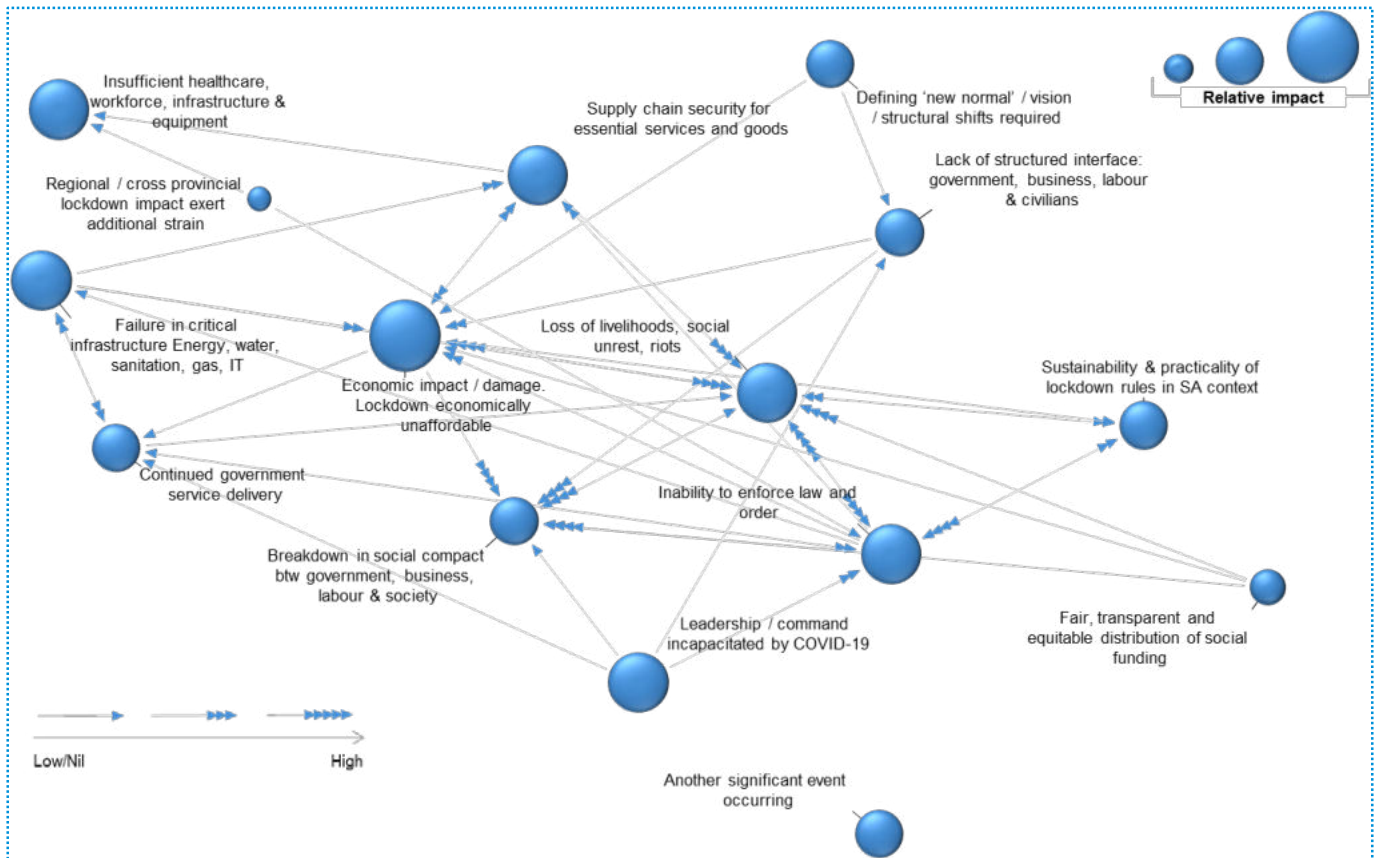
Figure 2: Causal linkages between discrete risks identified by participants through network theory
