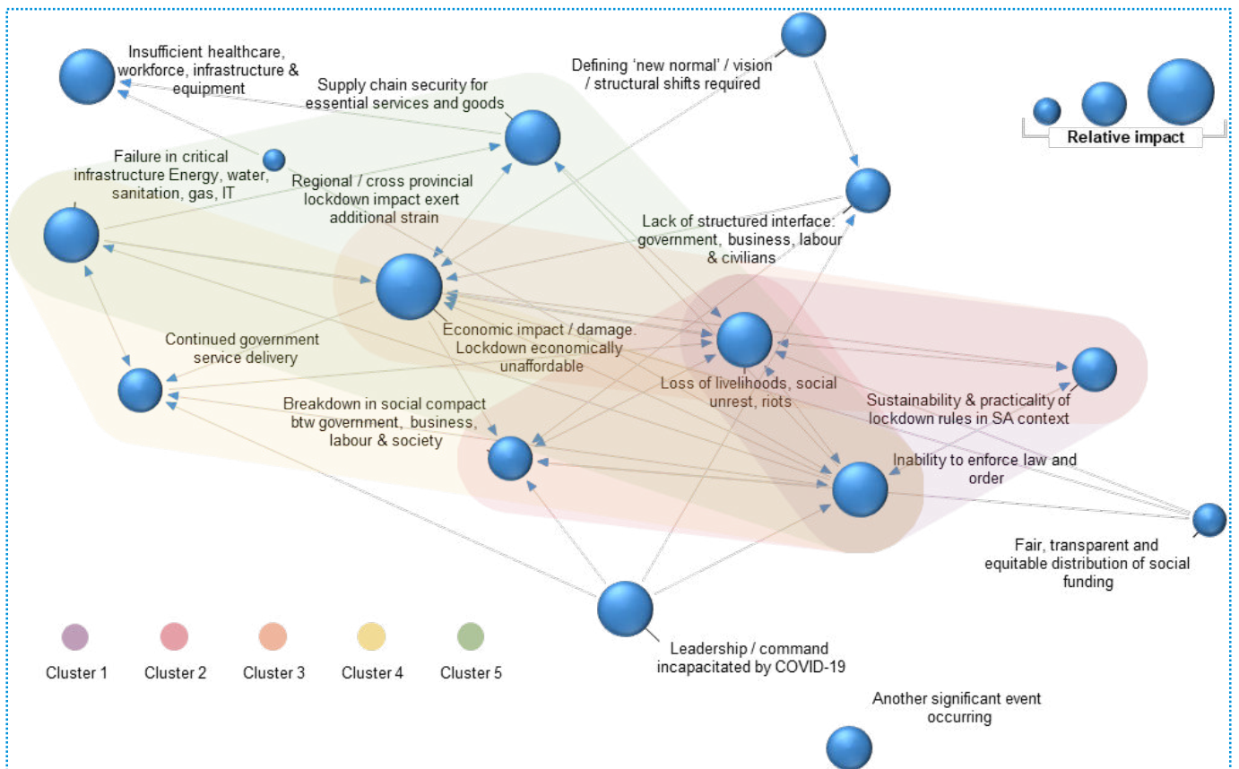
Figure 3: Clusters from network most expected to be encountered
